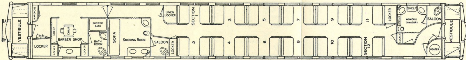
Cut out and plans of The Oriental Twelve Section Pullman Tour Sleeping Cars showing location of barber shop and men's shower bath as well as other features of interest.
