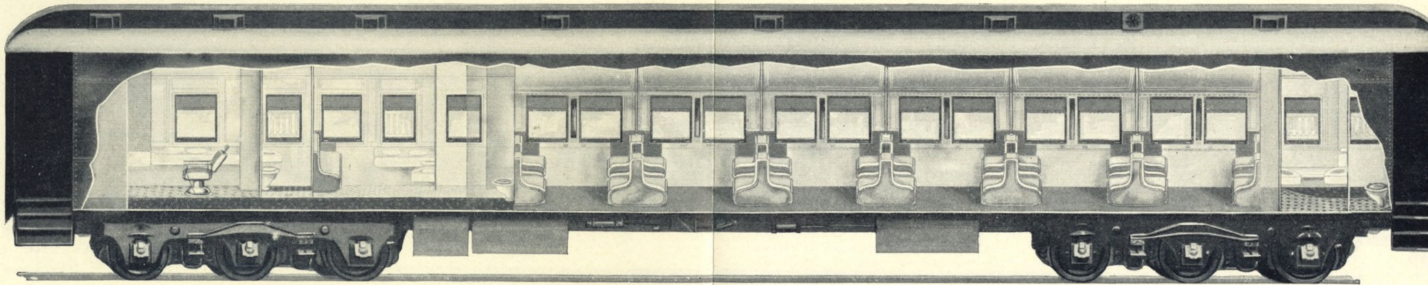
Cut out and plans of The Oriental Twelve Section Pullman Tour Sleeping Cars showing location of barber shop and men's shower bath as well as other features of interest.
