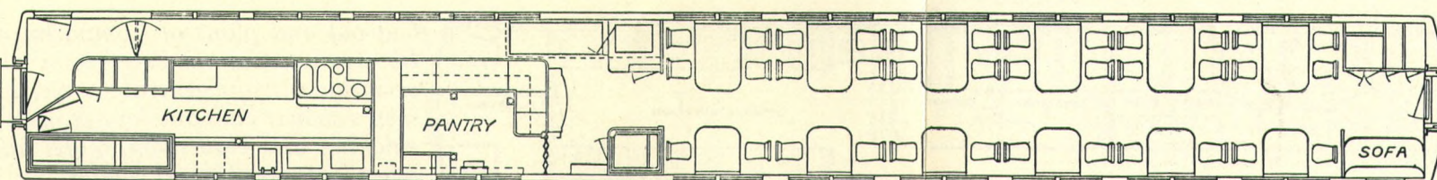
Cut out and plans of The Oriental Handsome Diners, seating 36 people showing lay out and details of construction.
